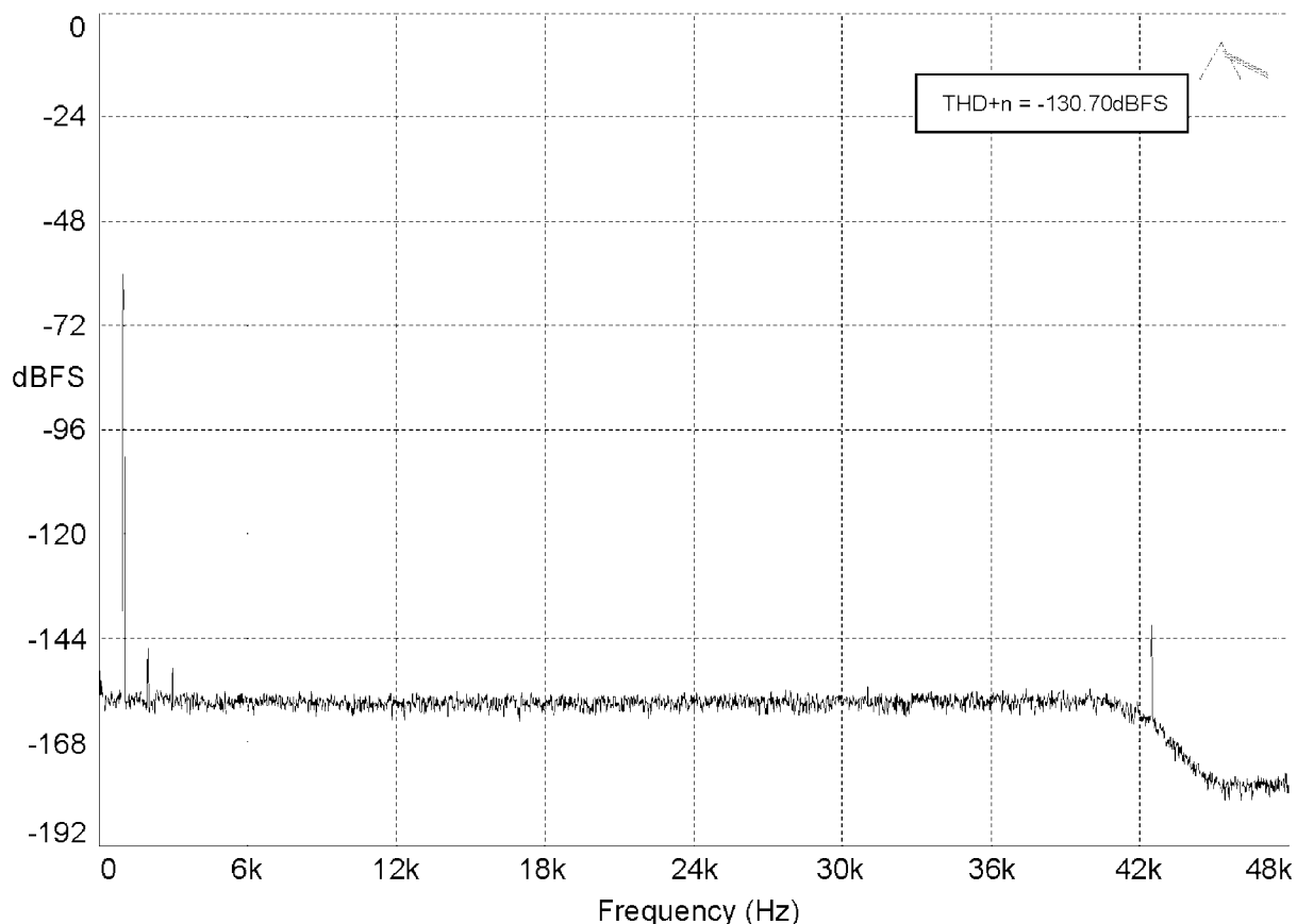
Figure 21: A-D mode Dynamic Range, at +28dBu sensitivity, 1kHz sine @ -60dBFS
