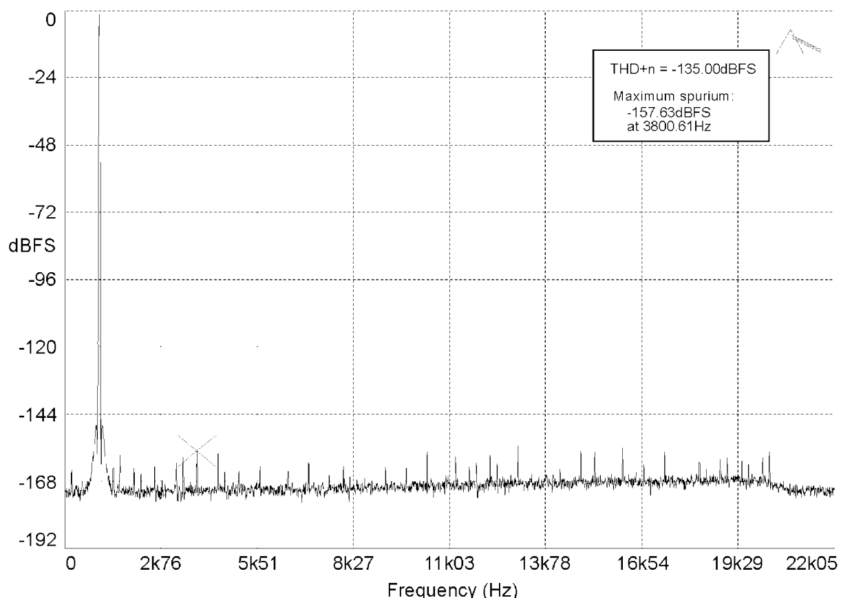
Figure 23: D-D SRC mode THD+n, 96kHz-to-44.1kHz, 1kHz sine @ 0dBFS
