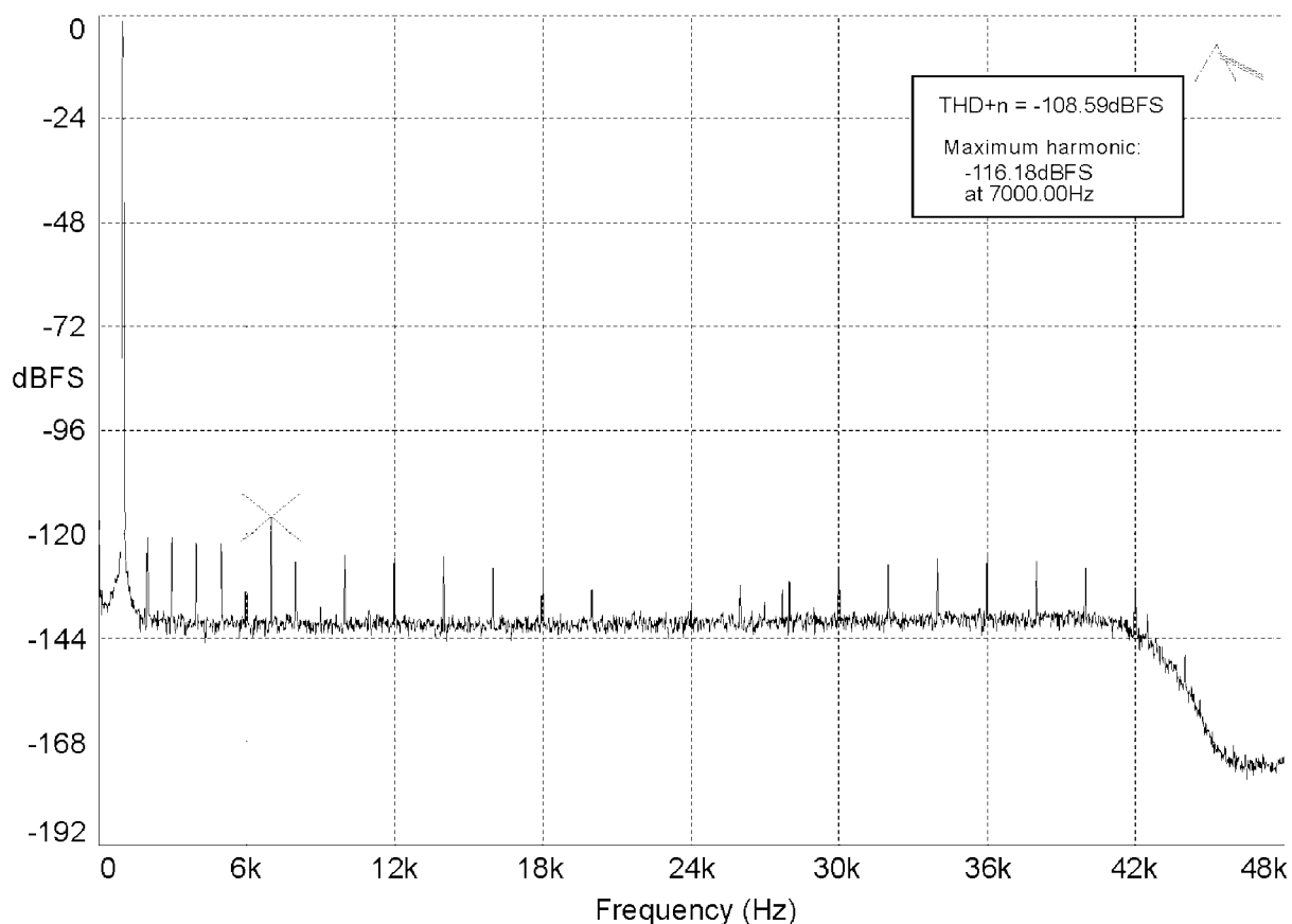
Figure 22: A-D mode THD+n, at +18dBu sensitivity, 1kHz sine @ -1dBFS
